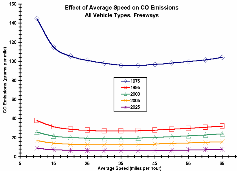
FIGURE III-1: Effect of Average Speed on CO Emissions for Freeway Facility types (adapted from Figure 28 of EPA’s Sensitivity Analysis of MOBILE6 , EPA420-R-02-035, December 2002)
